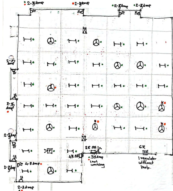
Existing Electrical Layout
