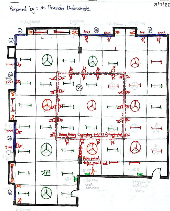
4 th Year Studio - Electrical Layout Proposal
